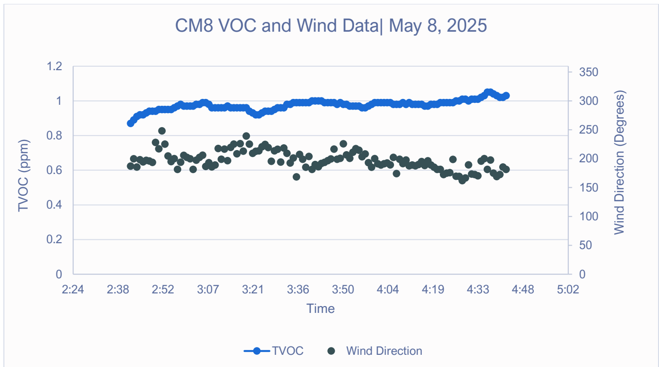
Figure 2 CM8 – Monroe Street tVOC and Wind Direction May 8, 2025, 2:42 AM to 4:42 AM
